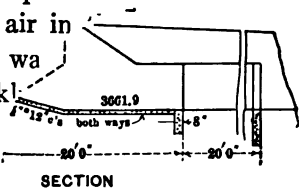
SECTION way, Fort Shaw Canal, Montana.
